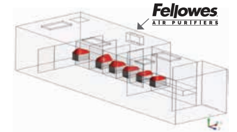
Contaminant Cloud With System Over Stalls
